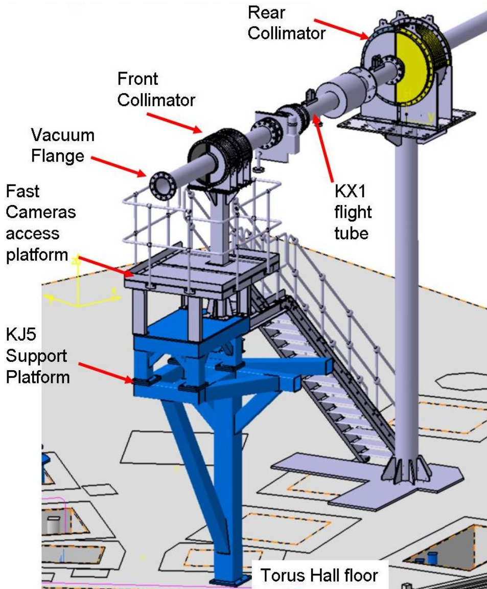
Figure 2.1 Tandem Collimators location
