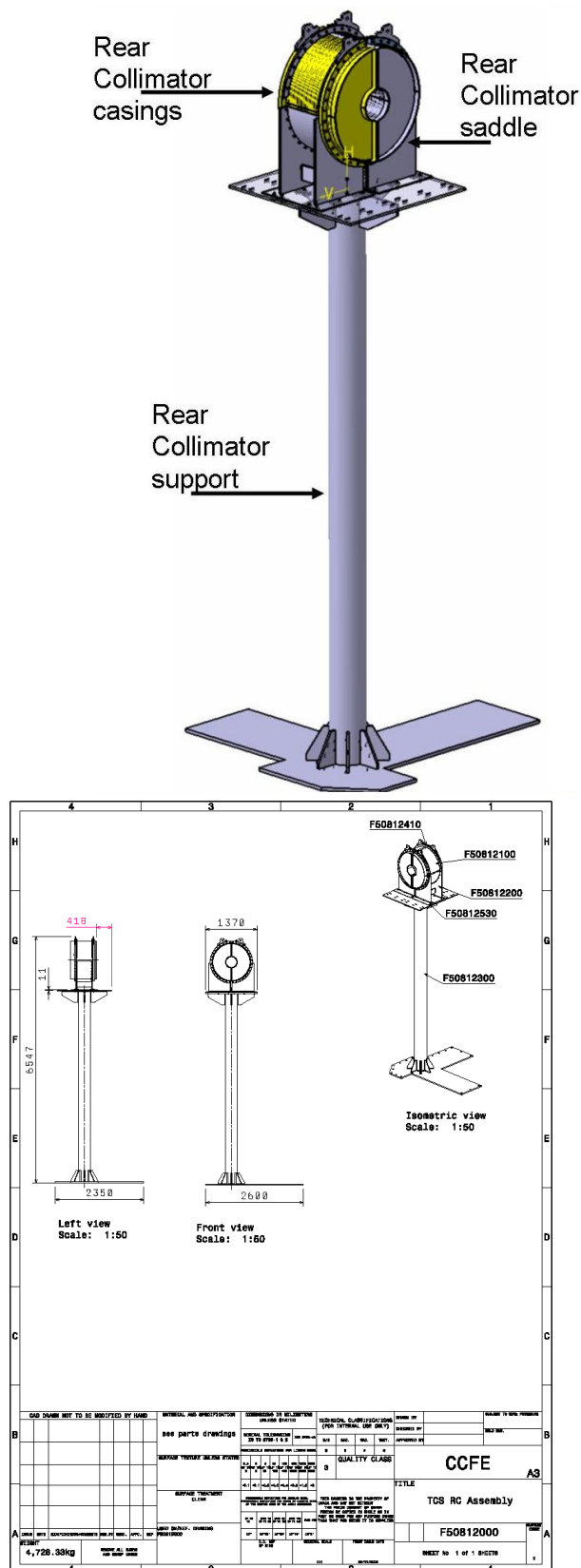
Figure 2.3 Rear Collimator
