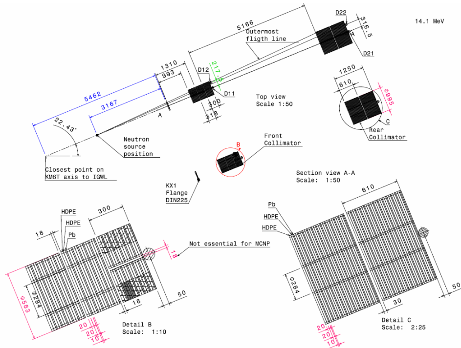
Figure 4.3- KM6T-TC configuration CONFIG-5 used for the Monte Carlo simulations
