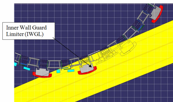
Figure 4.2 - Parasitic gamma-ray sources: IWGL's and their supports
