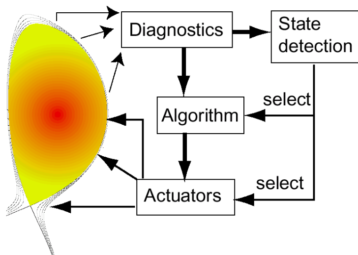
Figure 4.6-2 Plasma Feedback Control
